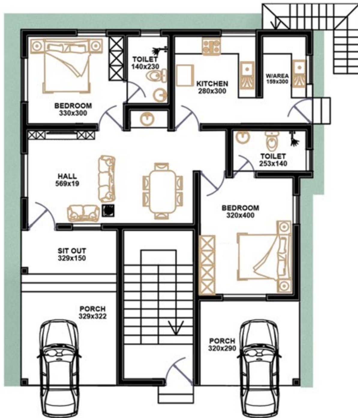
GROUND FLOOR AREA - 1276 SQ FT
