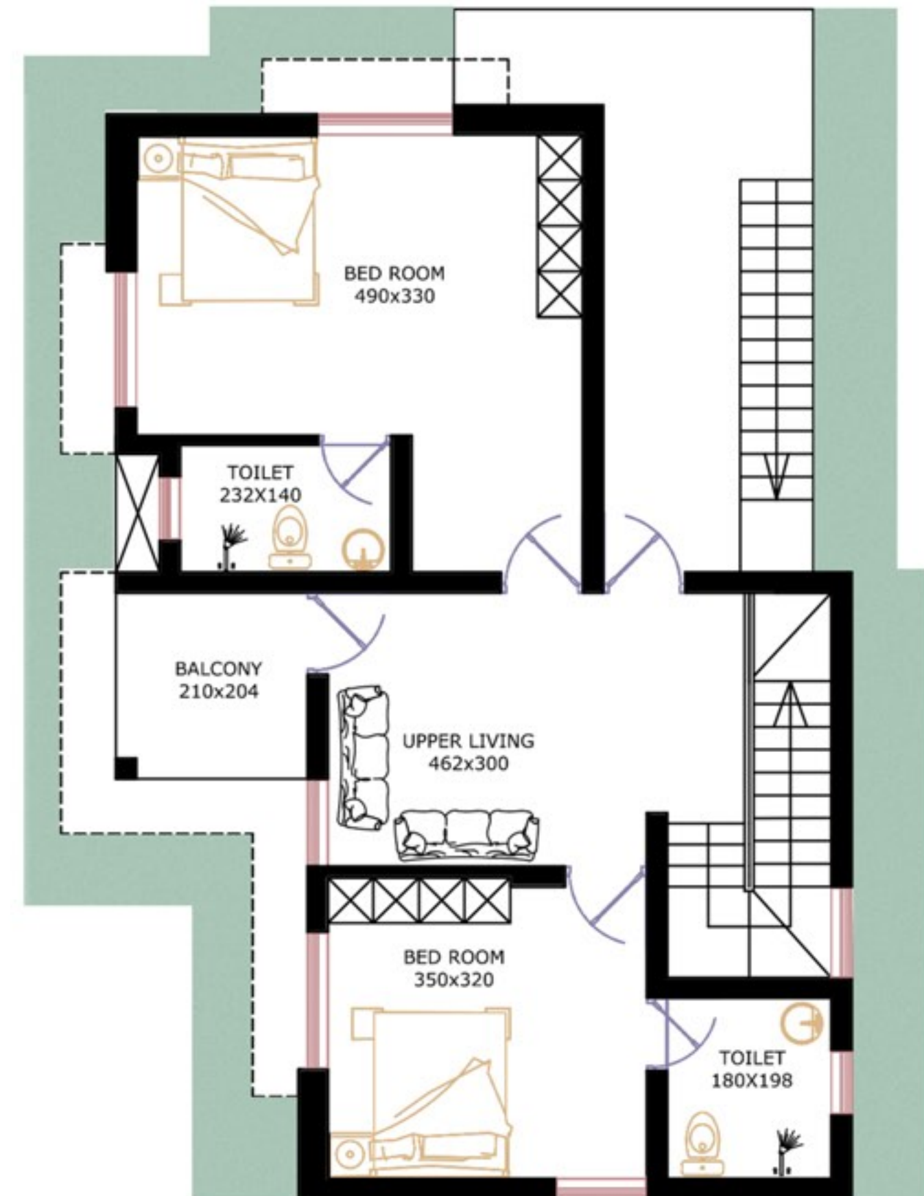
FIRST FLOOR Area - 774 SQFT
